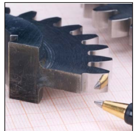
Figure 6 Near-mirror quality of a superfinished test gear.
