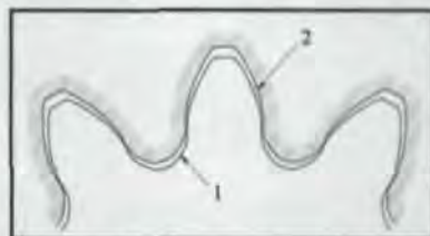
Fig. 8—Molding tool cavity profile definition; 1—the gear profile, 2—the cavity profile.
