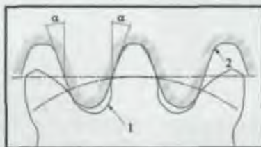
Fig. 7—Reversed "gear forms tool" rack-type tool profile generation; 1—the gear profile, 2—the tool profile.
