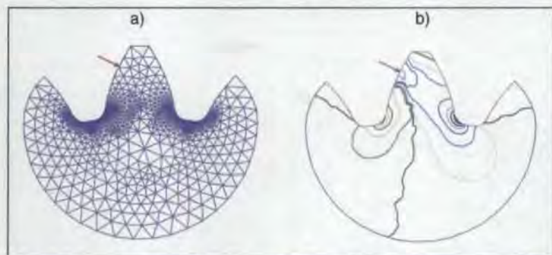
Fig. 1—The FEA gear tooth model: a) FEA mesh, b) stress isograms.
