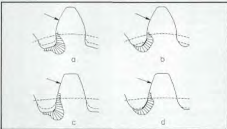
Fig. 4—Bending stress concentration for the balanced, traditionally designed (standard tool parameters) gear pair. Dashed line is the form circle; dotted line is the trajectory of the mating gear tooth; thick line is the stress concentration area; a and b are the 12-tooth pinion profiles before and after optimization, respectively; c and d are the 41-tooth gear profiles before and after optimization, respectively.
